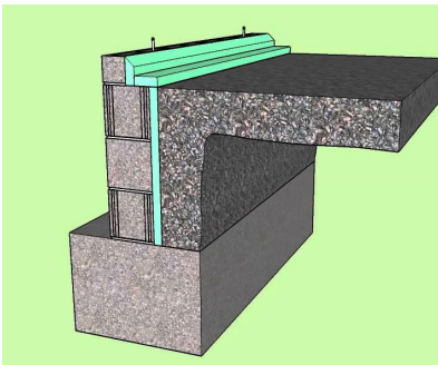
Stem wall slab insulation.
