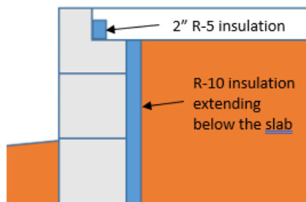
A diagram depicting the minimum requirements for stem wall slab insulation
